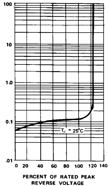
FIG. 4: TYPICAL REVERSE CHARACTERISTIC
